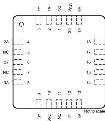
Figure 5-3. FK Package, 20-Pin LCCC (Top View)
